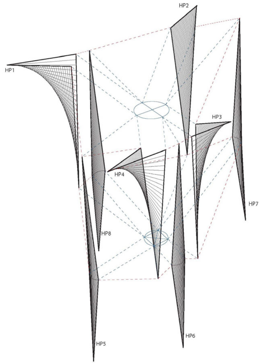
Exploded Axonometry of the central column _Assembly of different Hyperbolic paraboloids _Interdependency of geometrical forms
